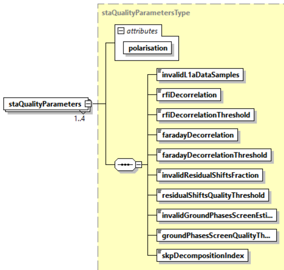
Fig.11 Input information DSR, staQualityParametersType
